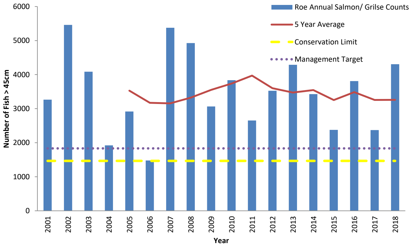
Fig.10 River Roe annual fish counts with 5 year average, management target and conservation limit.
