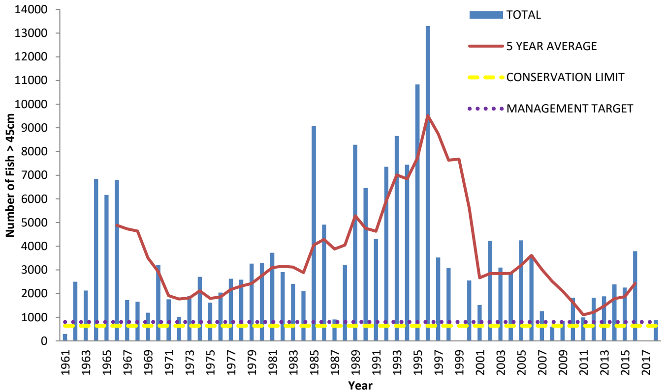
Fig.8 River Faughan annual fish counts with 5 year average, management target and conservation limit. NB: No Data for 2017
