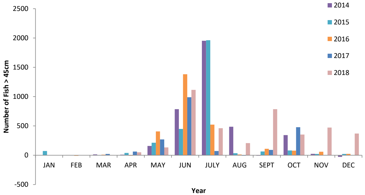
Fig.7 River Finn monthly fish counts. Negative counts represent kelts moving downstream.
