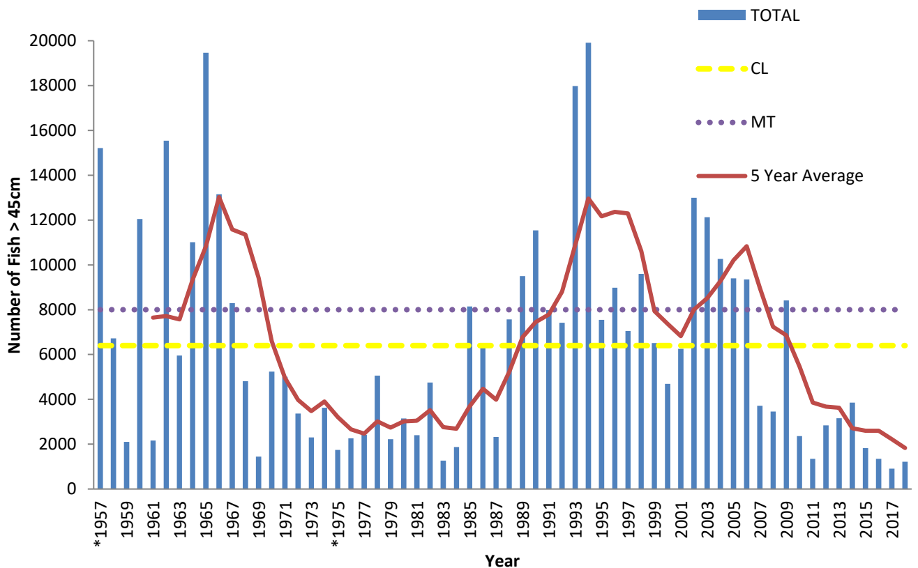
Fig.4 River Mourne annual fish counts with 5 year average, management target (MT) and conservation limit (CL).
