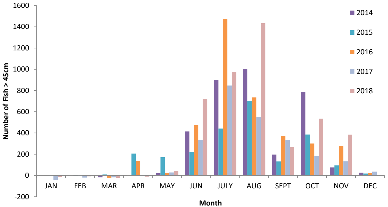
Fig.11 River Roe monthly fish counts. Negative counts represent kelts moving downstream.
